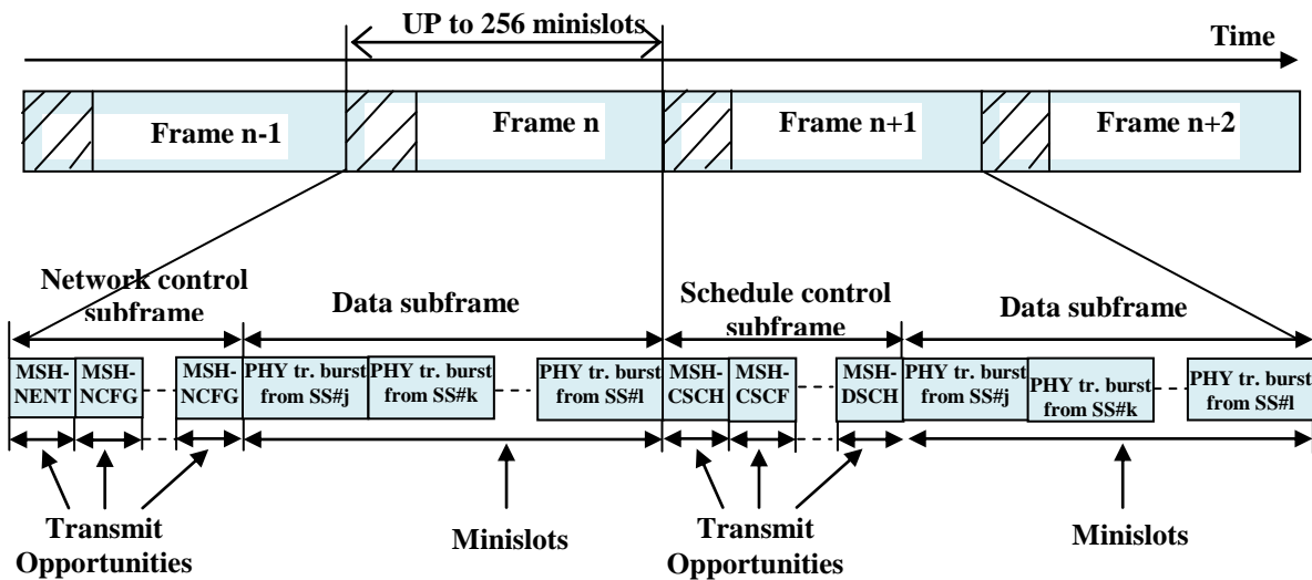
Fig.(2): frame structure in the mesh mode
