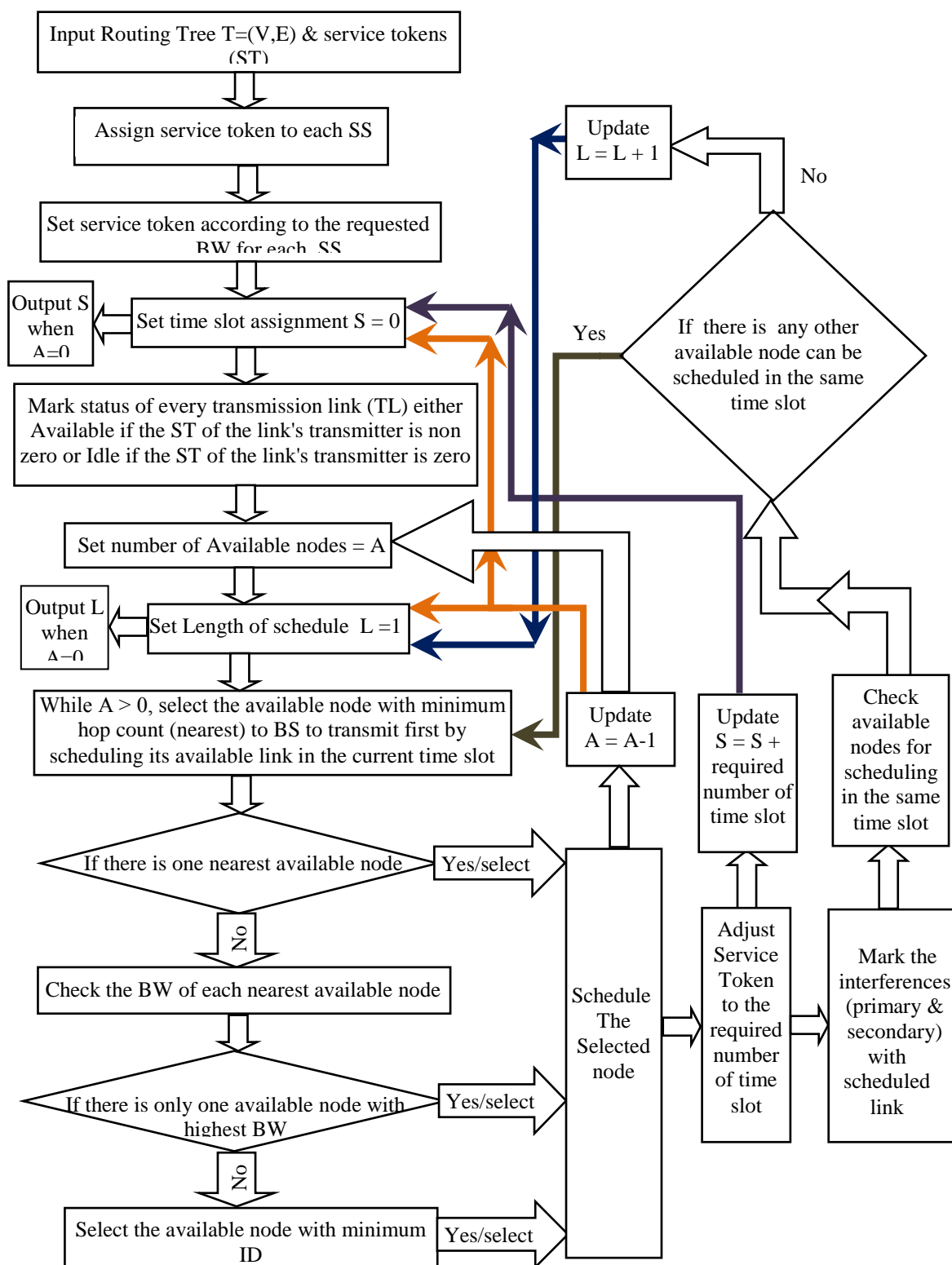
Fig.(8): Flow chart of the proposed scheduling algorithm
