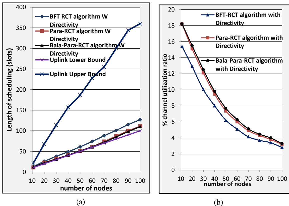
Fig. (12): shows the relationship between (a) the length of schedule and (b) channel utilization ratio against the number of nodes for BFT, Para and Bala-Para-RTCA with directivity when the traffic demand is unified and TR= 22.5 with uplink lower and upper bounds
