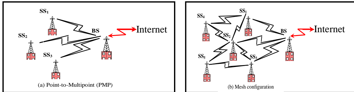
Fig.(1): WiMAX PMP network and mesh network
