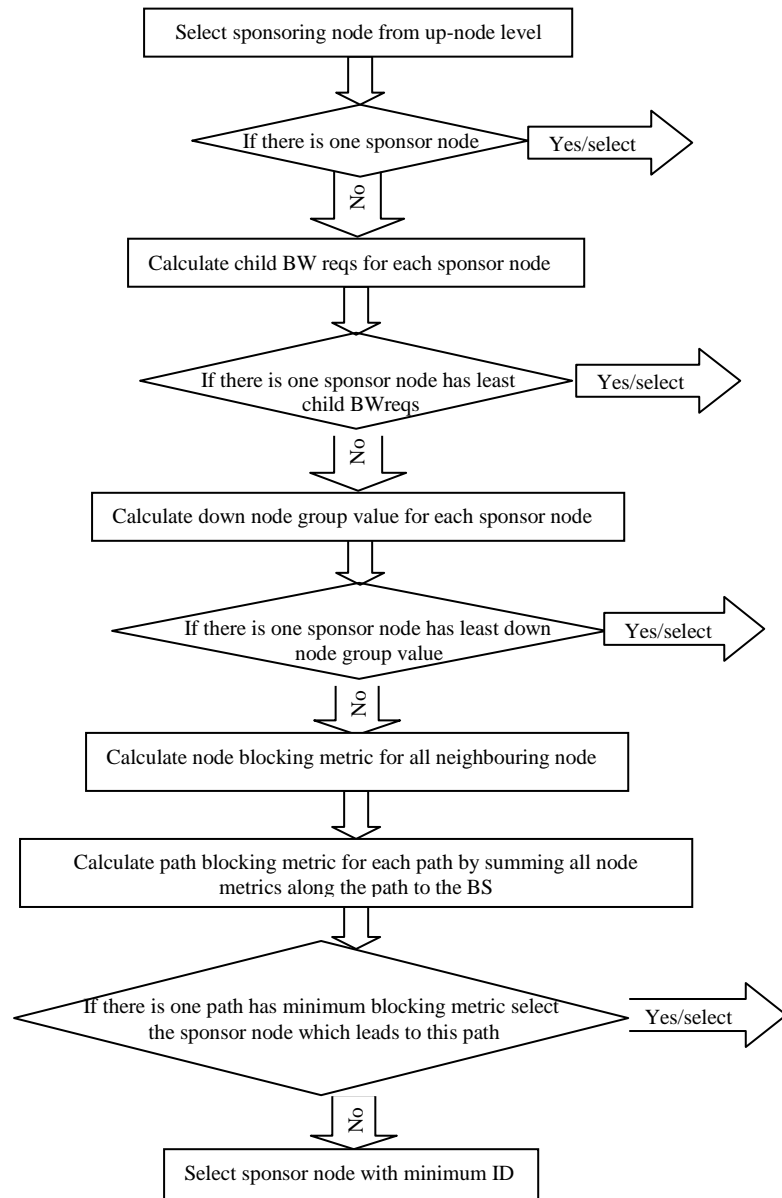
Fig. (5) Flow chart routing tree construction algorithm
