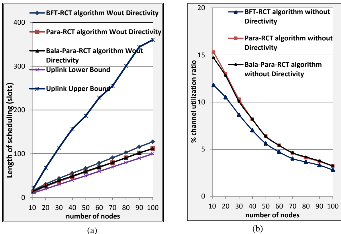
Fig. (11): shows the relationship between (a) the length of schedule and (b) channel utilization ratio against the number of nodes for BFT, Para and Bala-Para-RTCAs without directivity when the traffic demand is unified and TR= 22.5 with uplink lower and upper bounds
